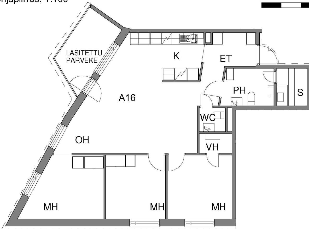
A16 (5.krs))
